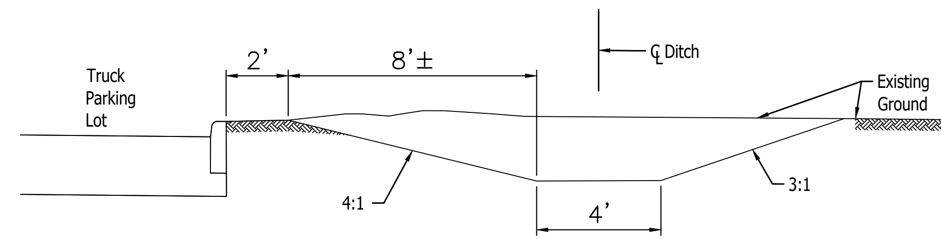
Ditch Typical Section Scale : None
